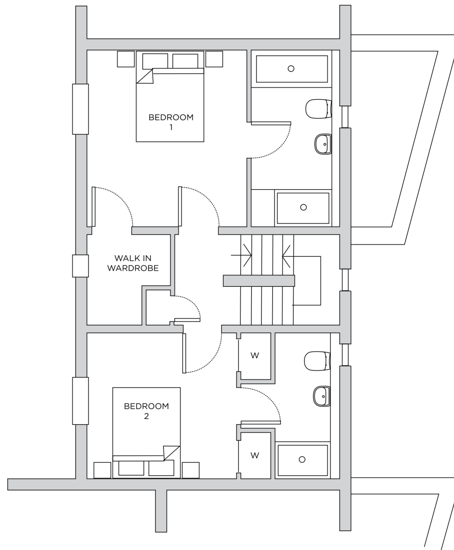
First Floor
